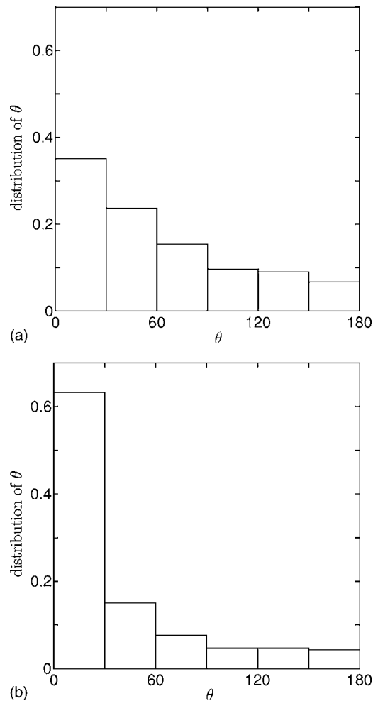
FIG. 4. The angle distribution of the advancing directions of particles for A=14 and U=1 . In the upper figure, the results for N=20 and in the lower figure, those for N=80 are depicted. For large N , the distribution concentrates near \theta=0 .
